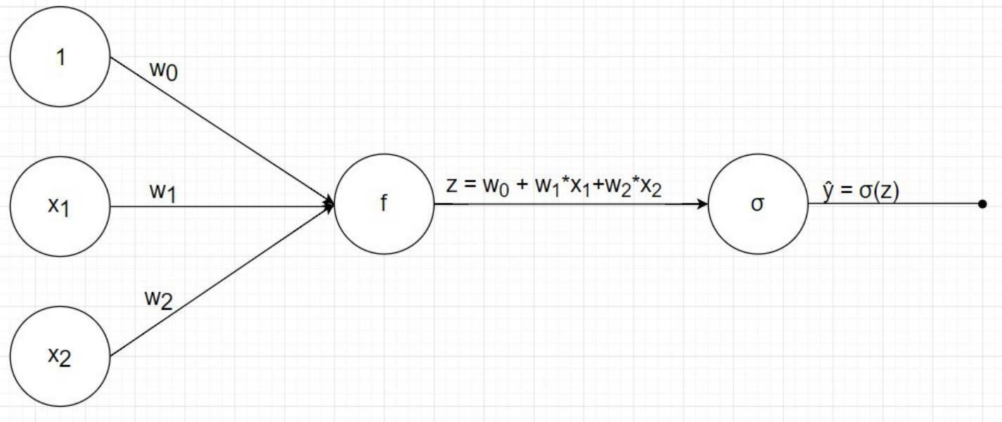
Flow chat of logistic regression model
